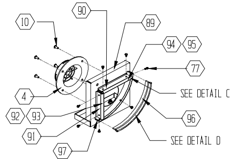
REACT PLENUM ASSEMBLY DETAIL
